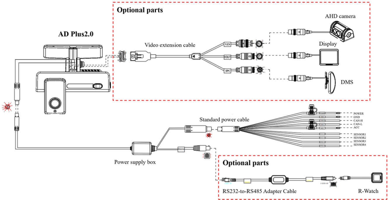
Figure 6: Dual Camera Connection overview – Discrete harness.
