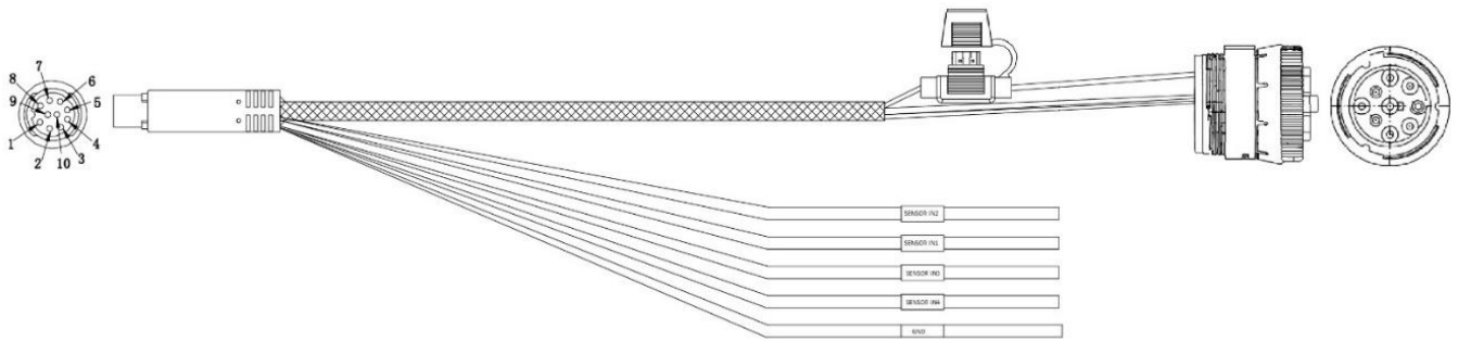
Figure 39: Power Harness: J1939 – 9Pin.
