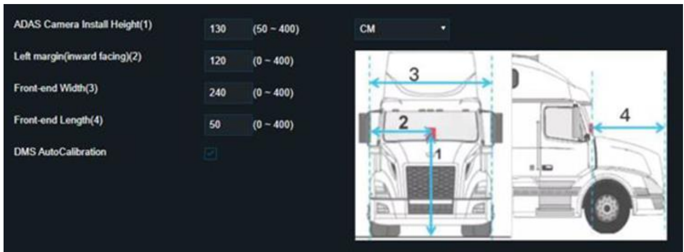
Figure 83: Screen for modifying the parameters outside the calibration.
