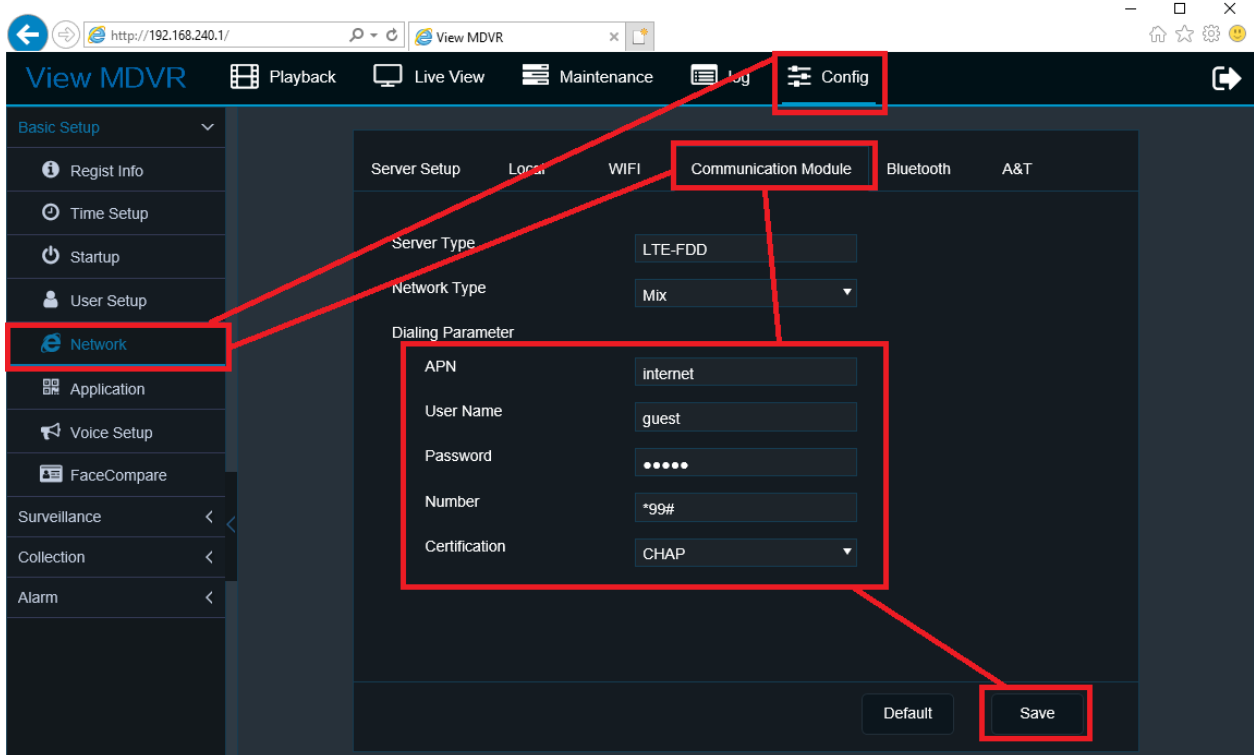
Figure 22: Setting up the APN.
