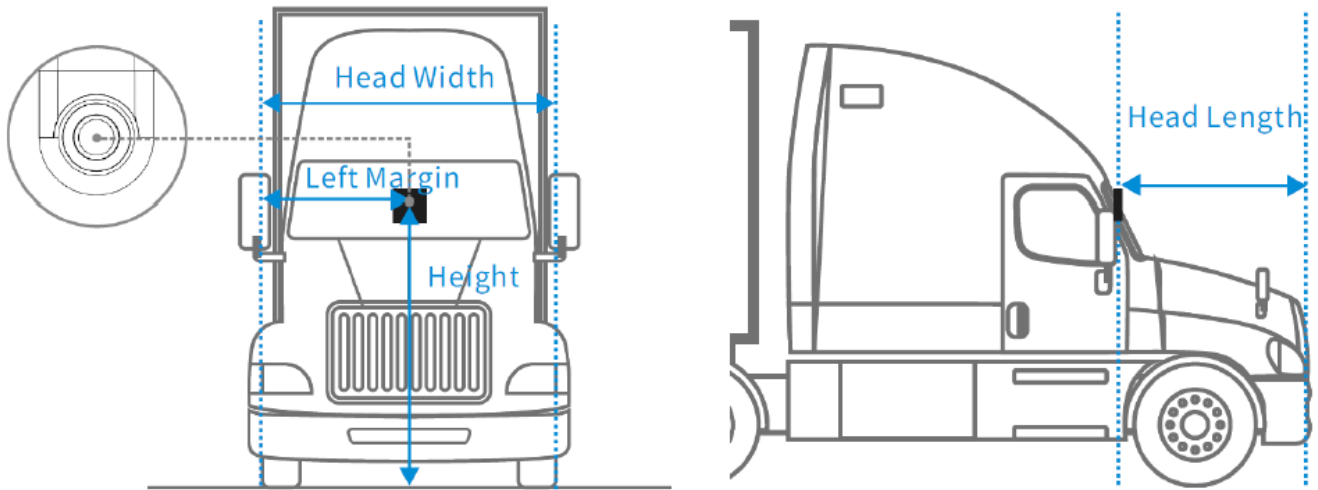
Figure 76: Vehicle measurements used during calibration.
