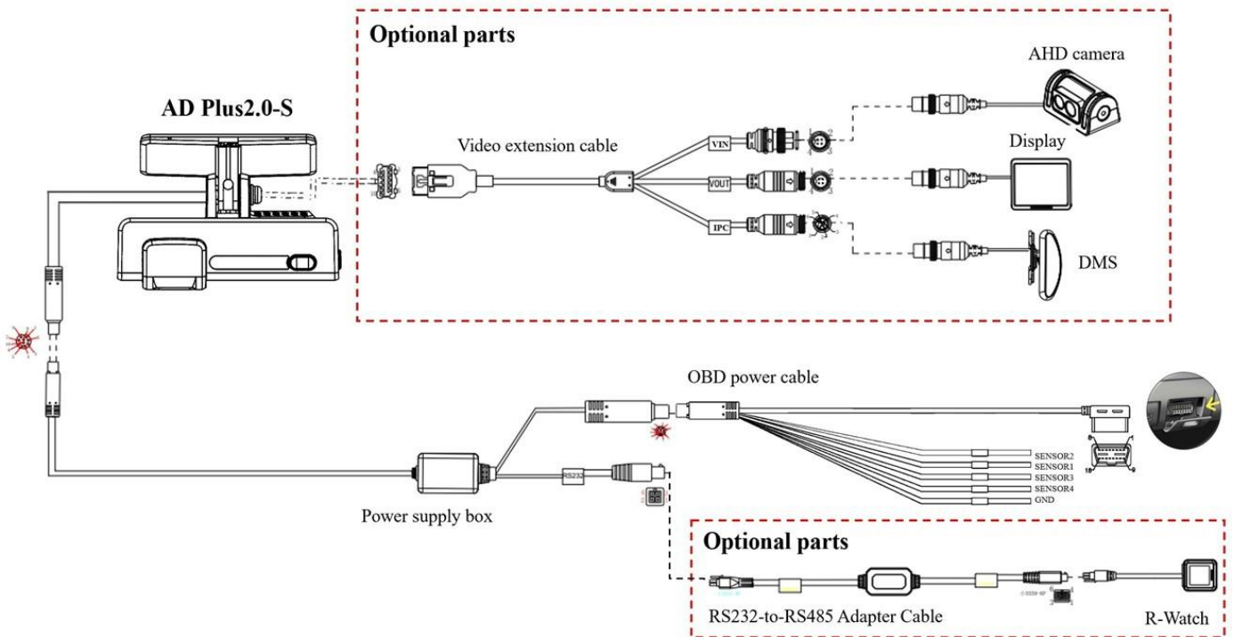
Figure 9: Single Camera Connection overview – OBDII harness.
