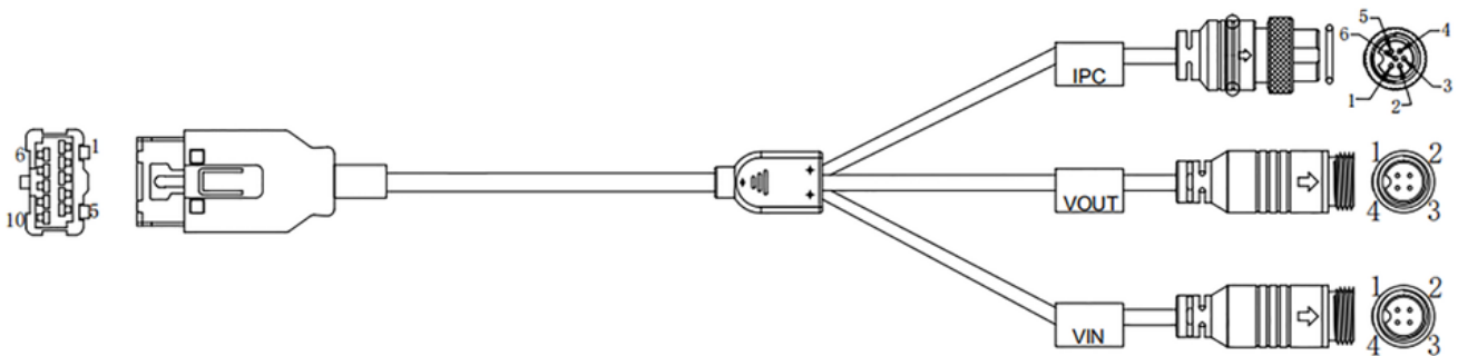
Figure 40: External camera harness.
