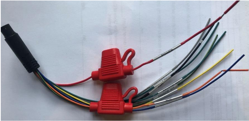
Figure 35: Power Harness: Discrete
